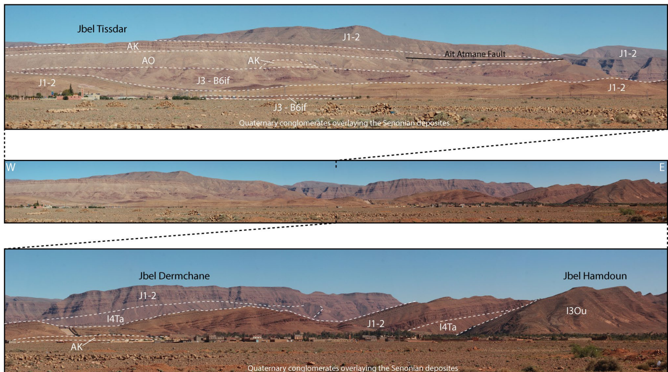
Fig. 6 Panoramic view of geosite ER1; AK: Cenomano-Truronian; AO: Cenomanian; B6if: Albian; J3: Bathonian; J1-2: Aalenian-Bajocian; I4Ta: Toarcian; I3Ou: Pliensbachian
