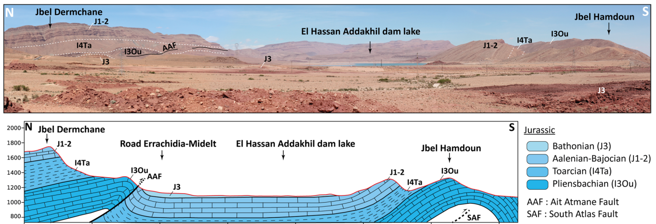
Fig. 15 Panoramic view and cross section illustrating the perched syncline structure (geosite ER5) between the South Atlas Fault and the Ait Atmane Fault
